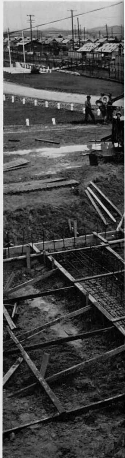
Pouring concrete footing
