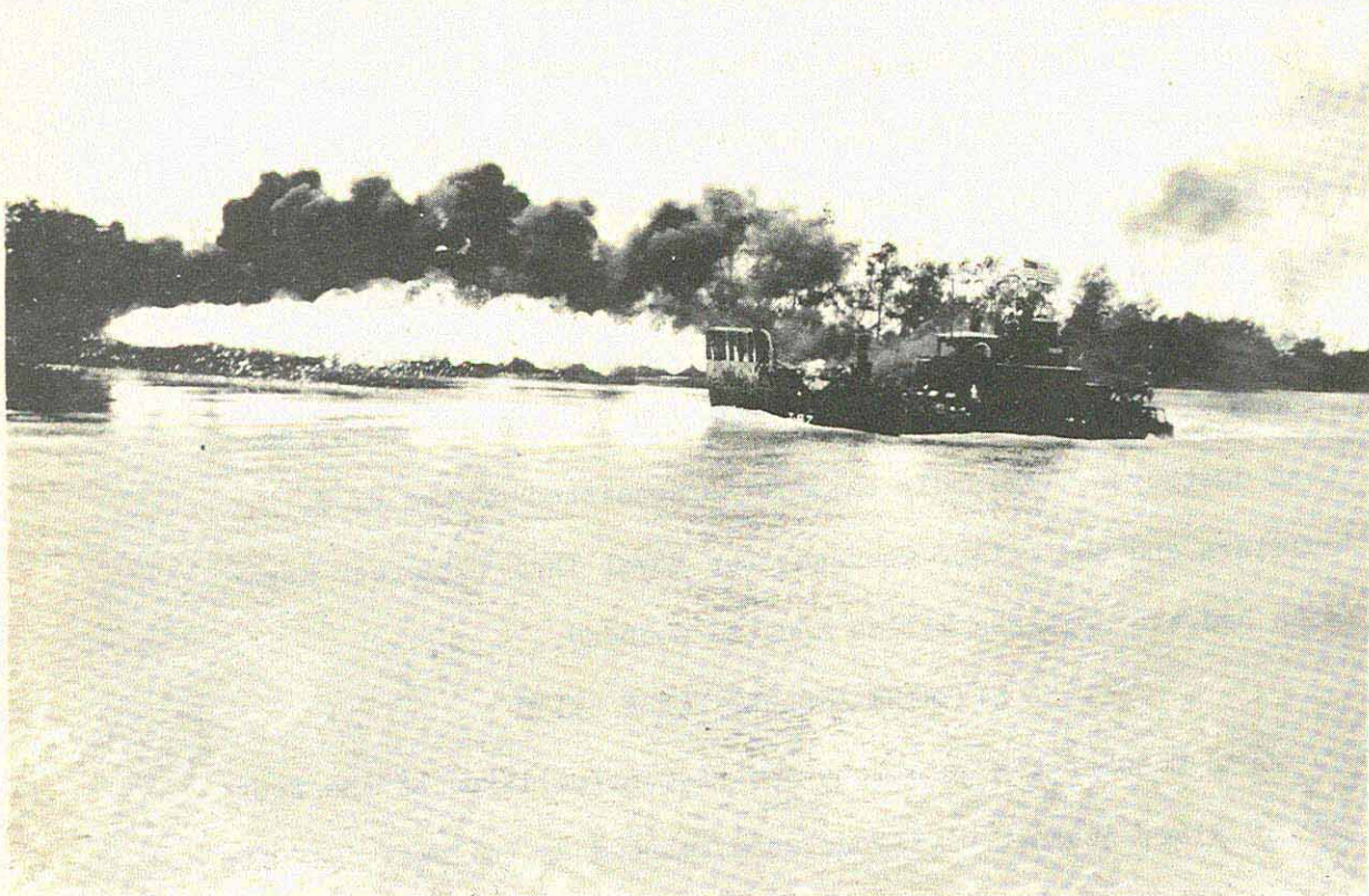
An ATC with a flame thrower (mounted in a U. S. Army APC carried in the well deck of the ATC) undergoes tests west of Dong Tam during October.
