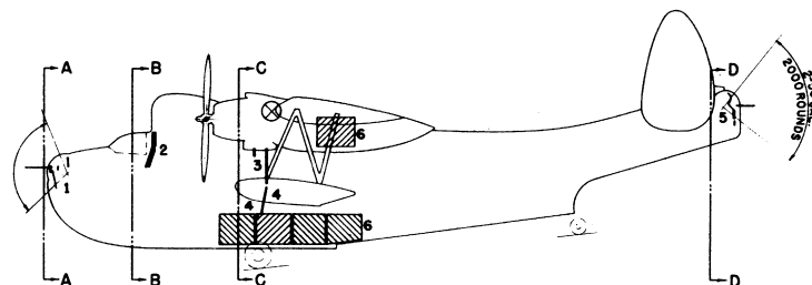
ARMAMENT & TANKS
