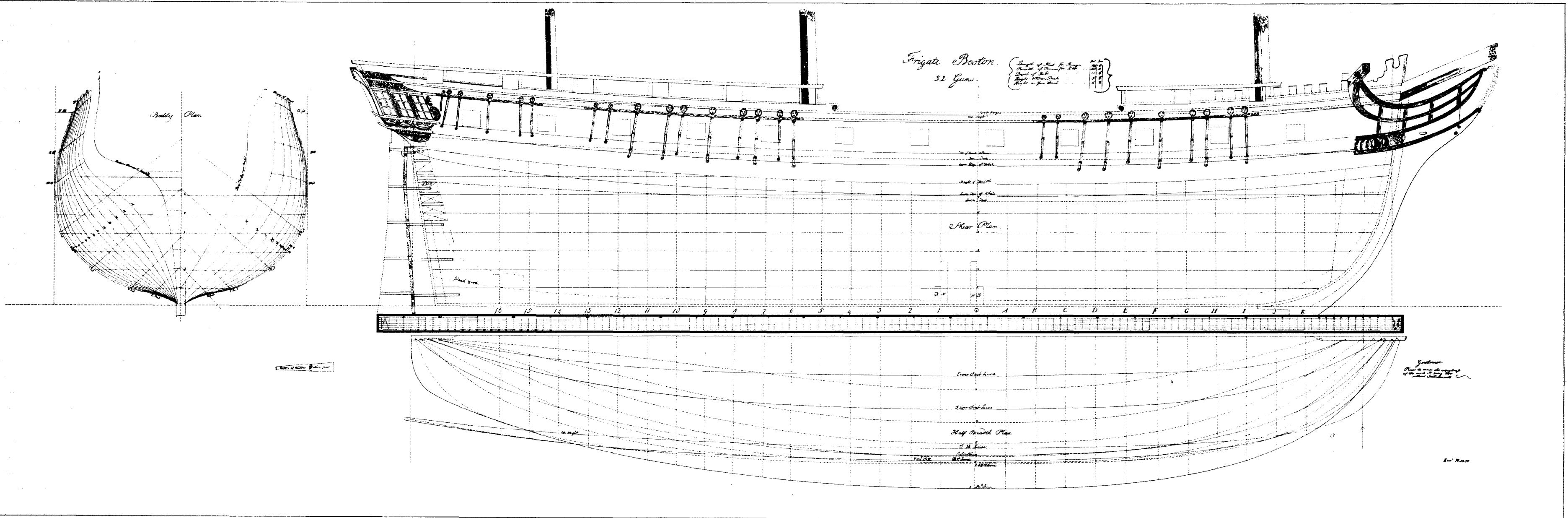
PLATE II. LINES OF THE UNITED STATES FRIGATE BOSTON.
