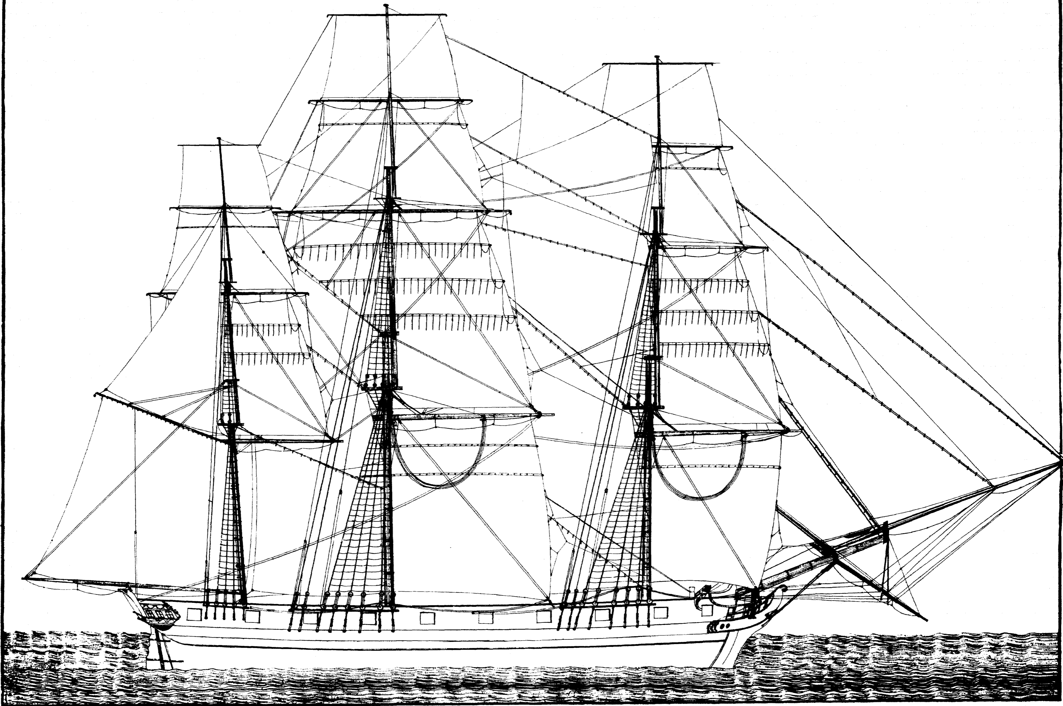
PLATE XI. SAIL PLAN OF THE UNITED STATES SHIP WASP.
