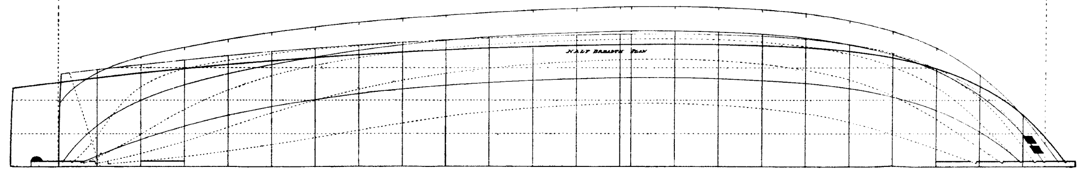
PLATE IX. LINES OF THE UNITED STATES SCHOONER (LATER BRIG) VIXEN
