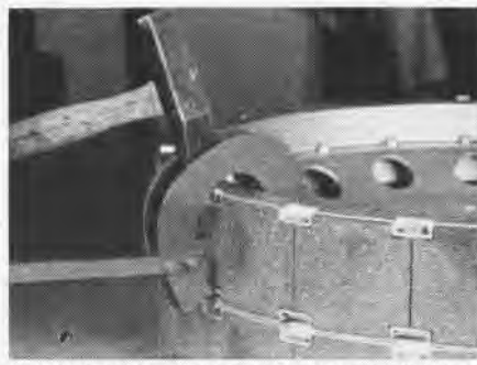
INSERTER TOOL ALLOWS ONE MAN TO DO WORK
